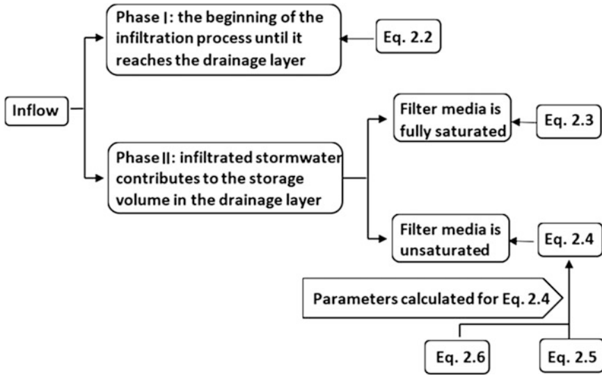
Fig. 2.5 The infiltration modelling process and equations used
