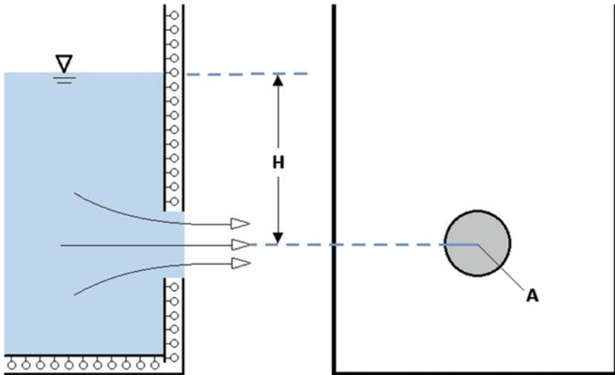
Fig. 2.11 Flow through a small orifice
