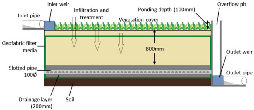
Fig. 2.2 The bioretention basin. a The bioretention basin at the site. b Cross-section
