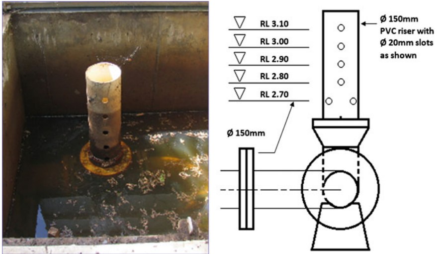
Fig. 2.10 The configuration of the PVC riser
