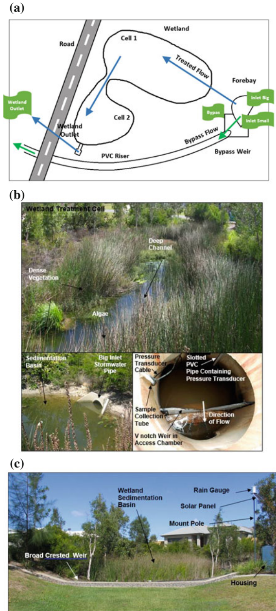
Fig. 2.6 The constructed wetlands. a Aerial view of the constructed wetlands. b The constructed wetlands at the site. c The bypass weir
