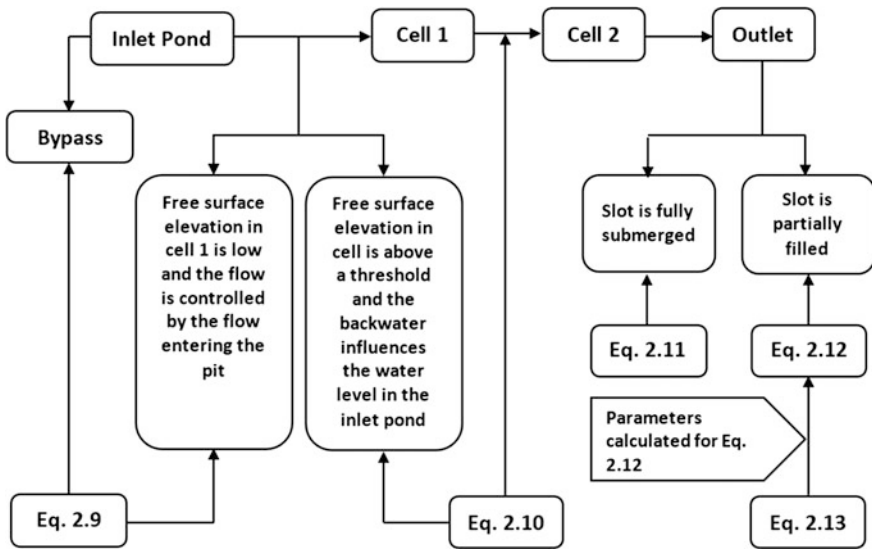
Fig. 2.13 Wetland modelling process and equations used
