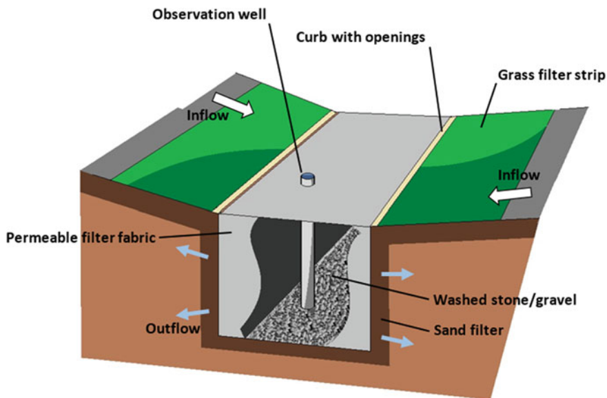
Fig. 1.6 Typical infiltration trench
