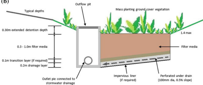
Fig. 1.7 A typical bioretention basin. a A bioretention basin. b Cross section
