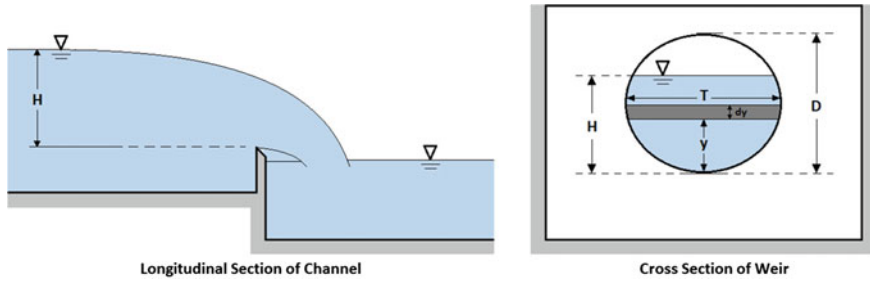
Fig. 2.12 Flow through a circular sharp-crested weir
