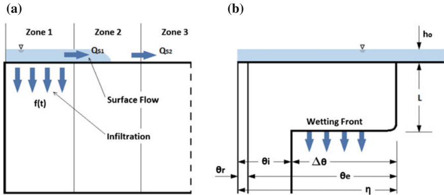
Fig. 2.4 Vertical soil column and Green-Ampt infiltration model
