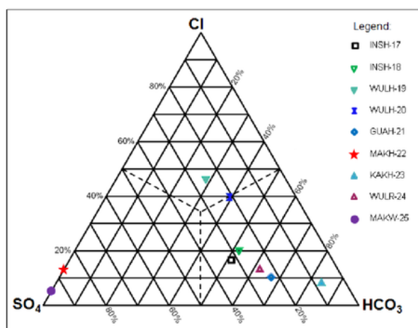
Figure 3: Ternary plot for Cl, SO 4 and HCO 3
