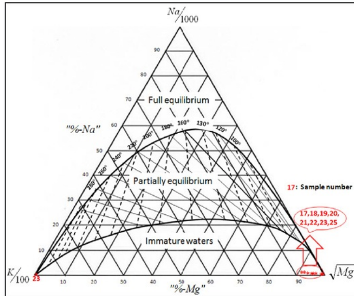
Figure 5: Ternary Na-K-Mg diagram.
