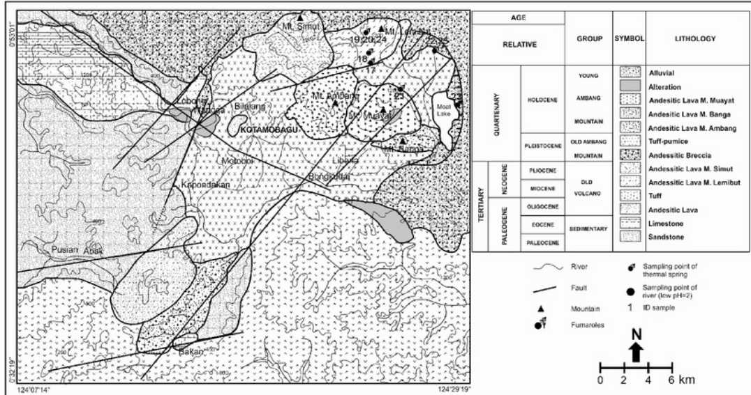
Figure 2: Geological Map of Kotamobagu (Modified from PT.PGE (2005)).
