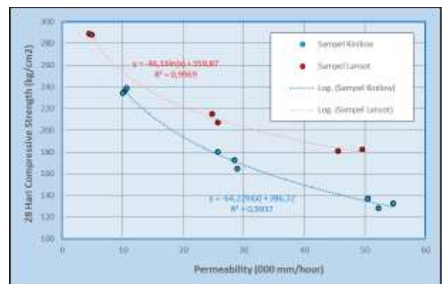
Fig. 2. Permeability versus 28 Days Compressive Strength
