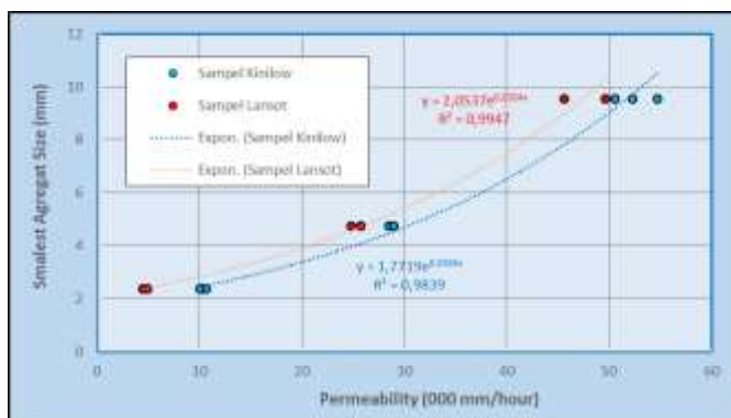
Fig. 3. Permeability versus Minimum Aggregate Size
