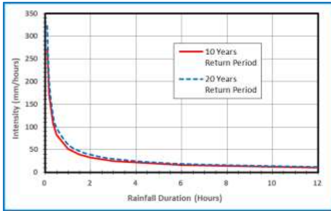
Fig. 1. Intensity-Frequency-Duration (IFD) Curve
