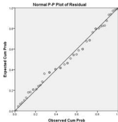
Gambar 4.1 Normality Residual Plot
