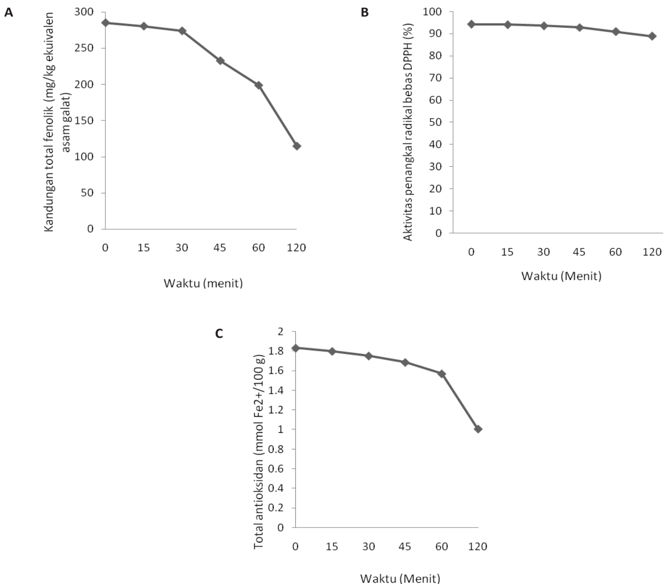
Figure 3. The effect of heating 100°C on change of total phenolic content (A), DPPH radical scavenger (B) and total antioxidant (C) of acetone extract (500 ppm) during 120 minutes heating.
