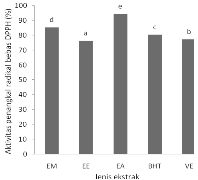
Figure 1. DPPH free radical scavenger activity of banana extract 500 ppm and standar samples. EM: methanol extract, EE: ethanol extract, EA: acetone extract, BHT: butylhydroxytoluene (200 ppm) and VE: tocopherol (200 ppm).
