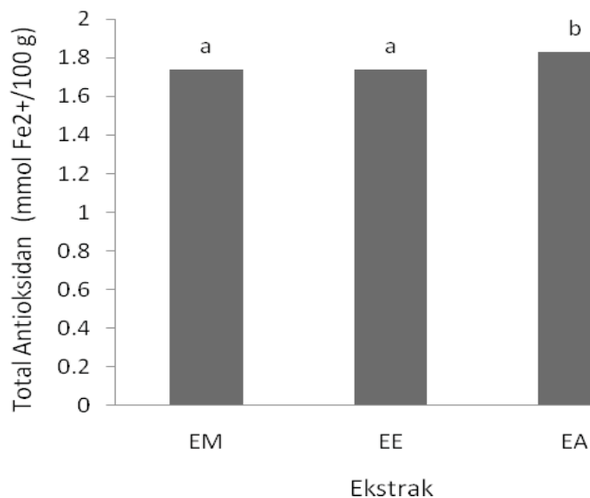
Figure 2. Total antioxidant content of goroho banana extract. EM: methanol extract, EE: ethanol extract and EA: acetone extract
