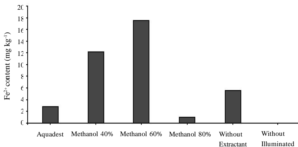
Figure 4. Ferrous concentration of water hyacinth leaves ( Eichhornia crassipessolms ) with aquadest and 40, 60 and 80% methanol solvents in the illuminated box on the photoreduction iron process.
