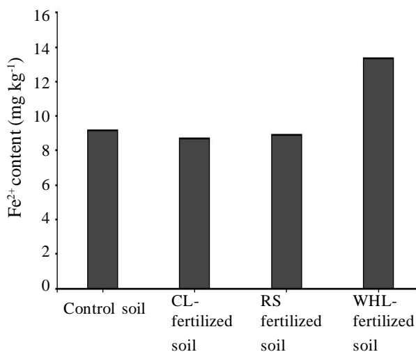
Figure 6. Ferrous concentration in green mustard of soil-fertilizer-extract of clove leaves (CL), rice straw (RS) and water hyacinth leaves (WHL) with 60% methanol in soil media and NPK fertilizer in the illuminated box on the photoreduction iron process.
