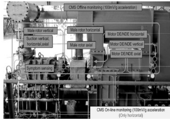
Fig. 2 Low methane compressor
