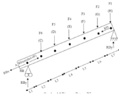
Gambar 4.8 Diagram Batang R7
