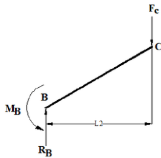
Gambar 4 Diagram benda bebas poros BC
