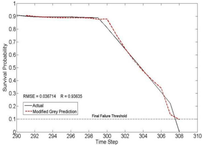
Fig.5. Modified grey prediction coupled with one-step-ahead technique.
