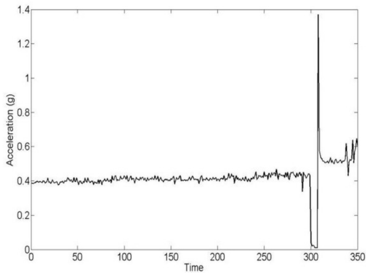
Fig.2. The peak acceleration data
