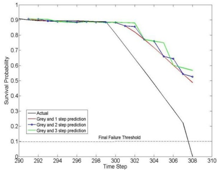
Fig.4. Grey predictions of machine's condition using 28 one-step-ahead, two-step-ahead, and three-step-ahead techniques.
