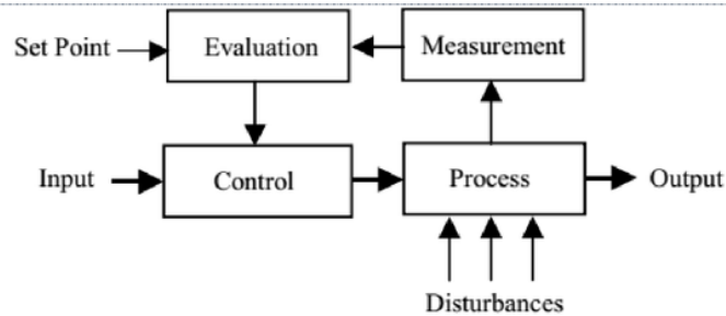
Figure 1. Four elements of a control system [3]
