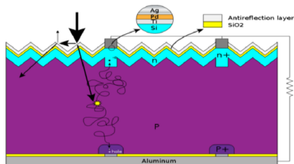
Figure 2. Silicon Solar Cell Structure [7]
