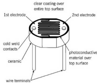
Figure 5. Light Dependent Resistor [13]
