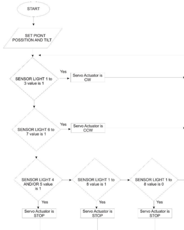
Figure 14. Flowchart of System Design
