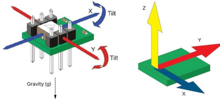
Figure 6. Principle of Accelerometer Sensor [14]
