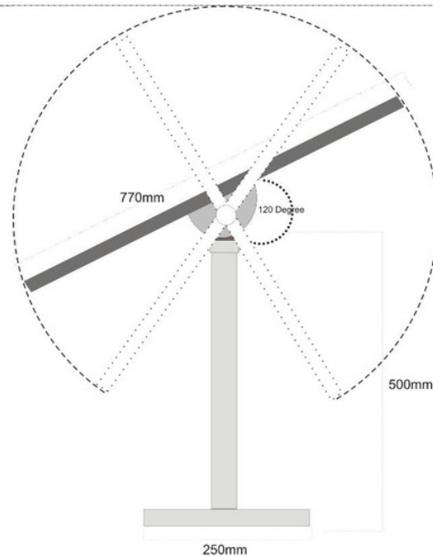
Figure 10. Prototype Side Design
