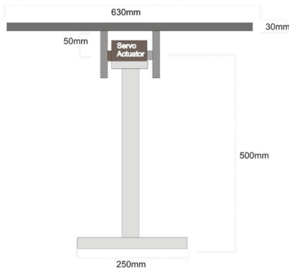
Figure 9. Prototype Front Design
