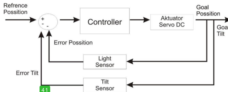
Figure 4. Block diagram Control System Solar Tracker
