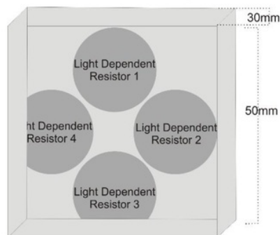
Figure 11. LDR Sensor Package
