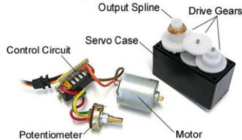
Figure 7. Servo DC Materials [17]
