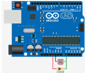
Figure 12. Wire of Arduino Uno with LDR Sensor
