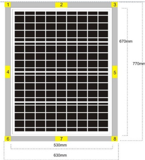
Figure 8. Modified Solar Panel Design
