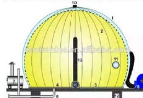
Gambar 2 sketsa beserta keterangan biogas storage
