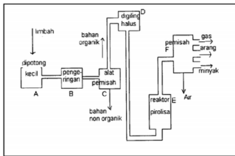
Gambar 1 Proses pirolisa
