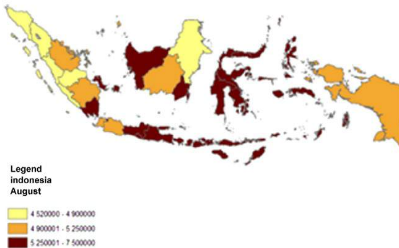
Fig. 16. Solar irradiation map by province in Indonesia on August.
