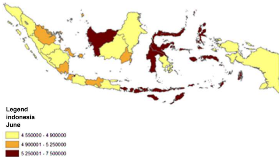
Fig. 14. Solar irradiation map by province in Indonesia on June.
