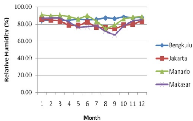
Figure 2(c) Typical relative humidity for four cities
