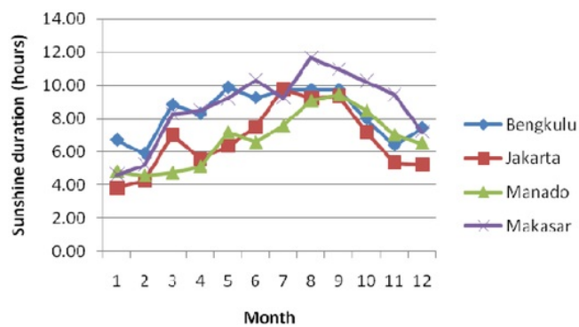
Figure 2(a) Typical sunshine duration for four cities
