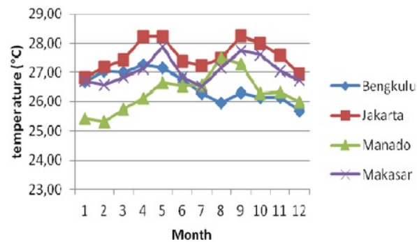
Figure 2(b) Typical temperature for four cities
