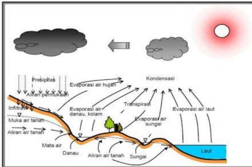
Gambar 2. Siklus Hidrologi Sumber : https://poetraffic.wordpress.com
