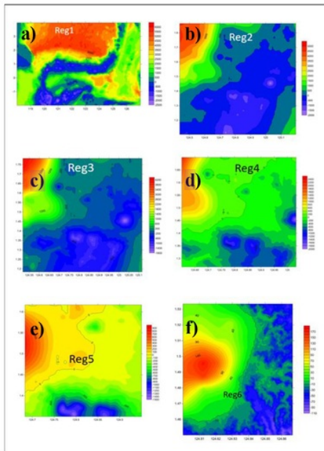
Gambar 4. Pembagian area simulasi tsunami domain model 1 sampai 6. a) Region 1 (1850 m); b) Region 2 (616,67 m); c) Region 3 (205,56 m); d) Region 4 (68,52 m); e) Region 5 (22,84 m); f) Region 6 (7,62 m)
