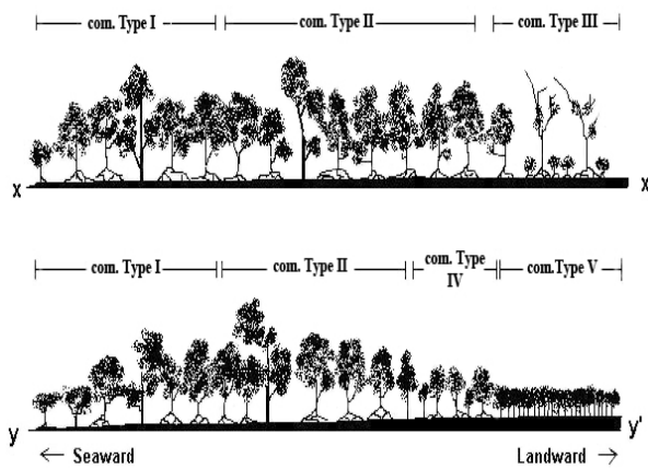
Figure 7. Profile diagrams of the recognized communities along transects x-x' and y-y' as indicated in Figure 2.
