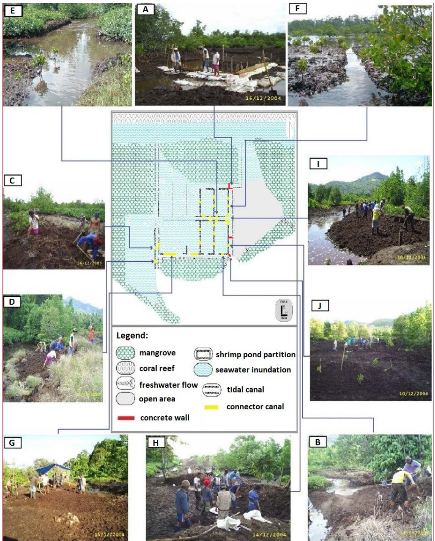
Figure 3. Physical changes to restore the hydrological condition.
