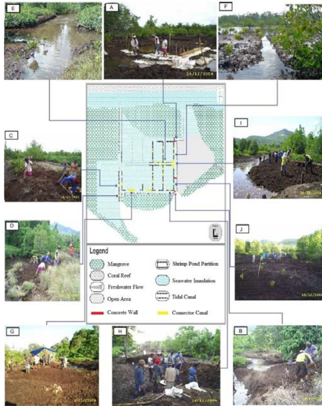
Figure 3. Physical changes to restore the hydrological condition.
