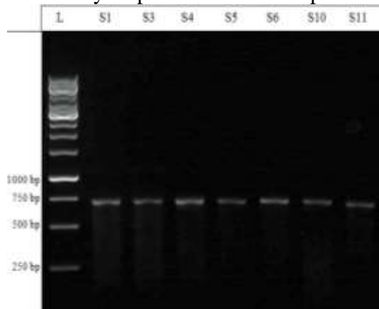
Figure 1. CO1 gene amplification of cuttlefish samples from Manado Bay and Lembah Strait on 1% agarose gel. L is GeneRuler, Thermo Scientific as marker. S1-S11 is sample numbers.
