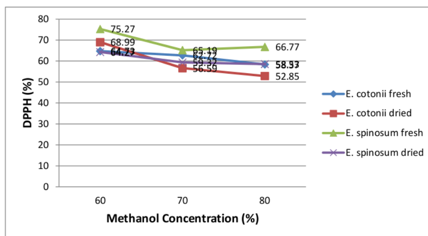
Figure 02. DPPH content
