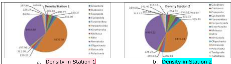
Figure 2. Density Meiofauna at Station 1 and Station 2.
