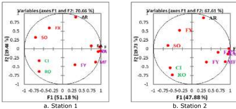
Figure 4. Circular correlation between variables on the main axis (F1 and F2).
