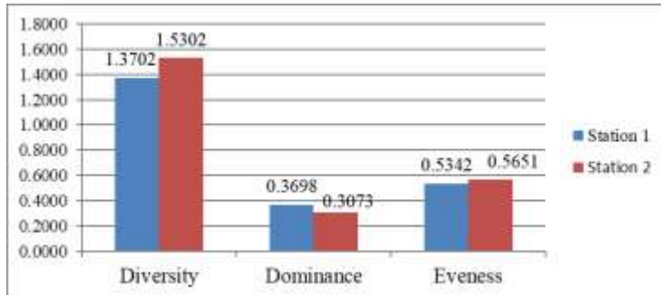
Figure 3. Index of diversity, dominance, and evenness.
