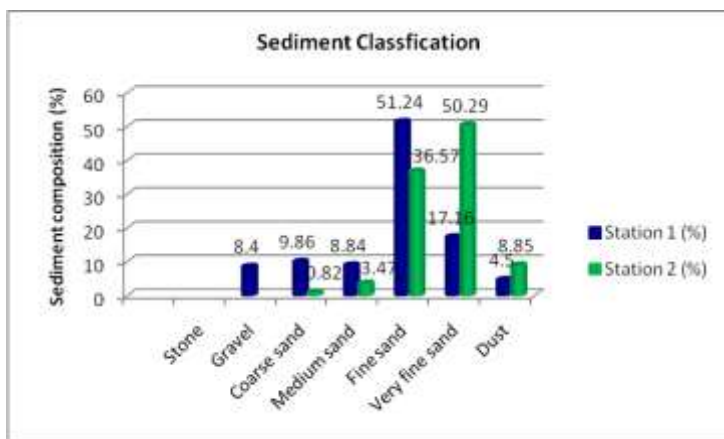
Figure 6. Sediment composition in station 1 and station 2.
