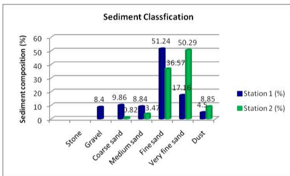
Figure 6. Sediment composition in station 1 and station 2.
