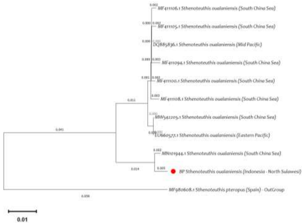
Figure 3. Phylogenetic tree of S. oulaniensis
