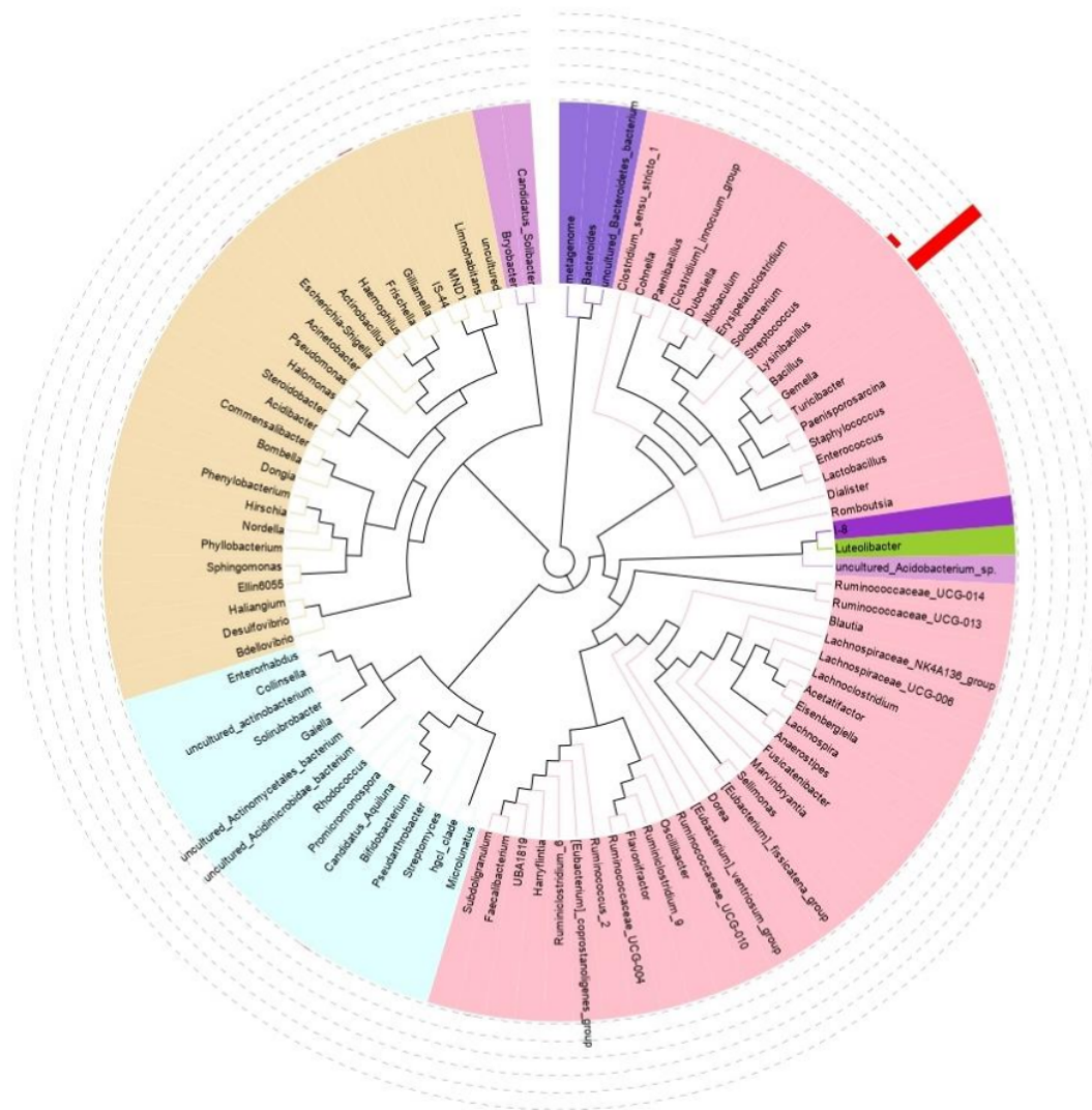
Figure 3. Genus evolutionary tree by using NJ methods. Red bars indicate the relative abundance of the taxa. Different colors of the branches represent different phyla. Relative abundance of each genus in each group is displayed outside the circle
