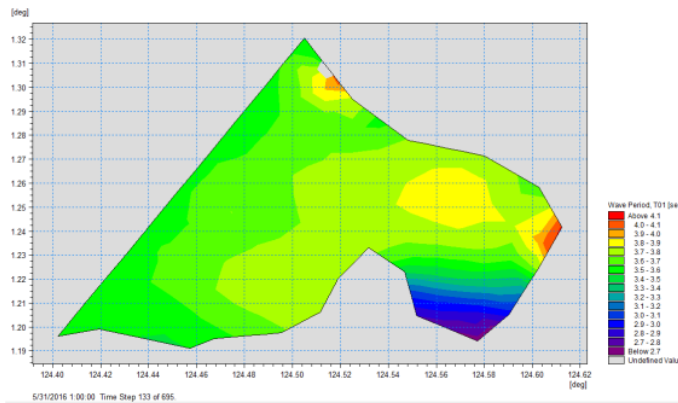
Figure 10. Wave Period distribution (T) at May-June period simulated using MIKE21 SW model
