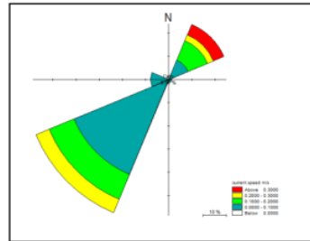
Figure 6: Current rose data 25 Nov-14Dec 2016
