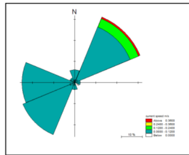
Figure 8: Current rose data 25May-23June 2016
