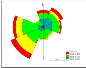
Figure 5: Current rose simulation 25 Nov-14Dec 2016
