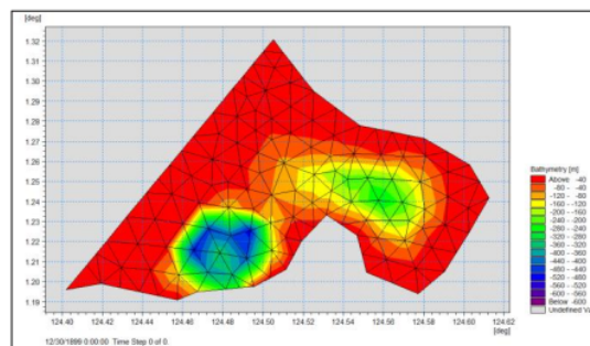
Figure 2. Unstructure Mesh and Bathymetry
