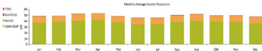
Fig. 3. The monthly average production based on the proposed hybrid power system in Miangas Island.
