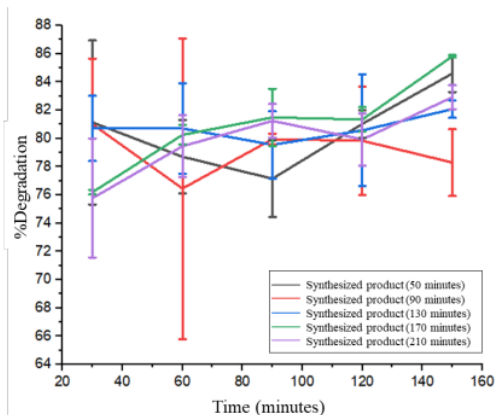
Figure 6. Effect of contact time on photocatalytic degradation of MB dye
