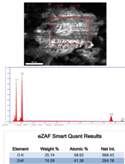
Figure 2. EDS data of synthesized product
