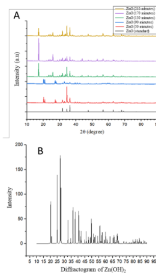
Figure 1. Diffractogram patterns of (a) ZnO standard and synthesized ZnO with different microwave heating times of 50, 90, 130, 170, and 210 minutes (b) Zn(OH)_2 .
