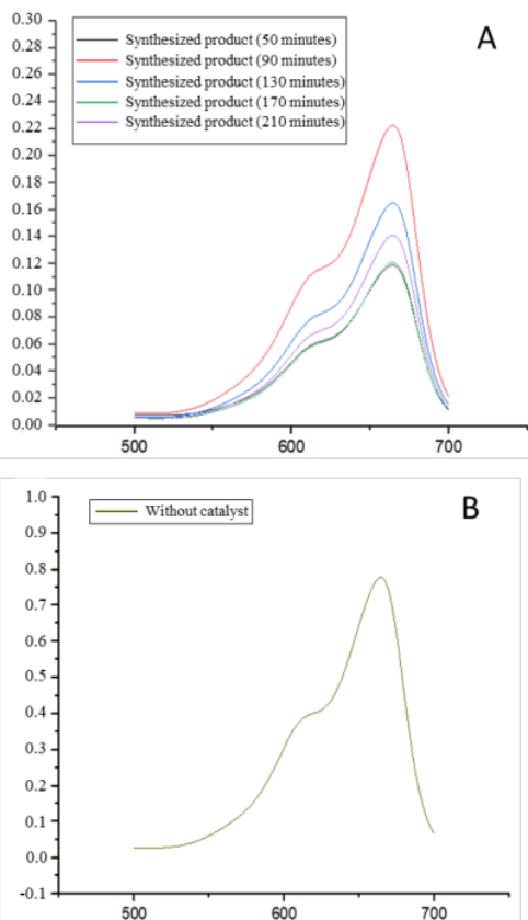
Figure 3. UV-Vis absorption spectra of MB solution (a) synthesized nanoparticles (b) without catalyst
