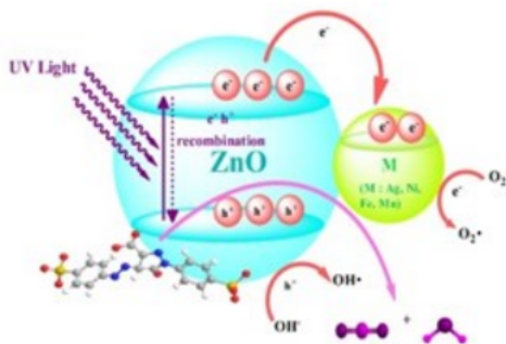
Figure 5. Photodegradation mechanism of MB dye by transition metal-doped ZnO [25]
