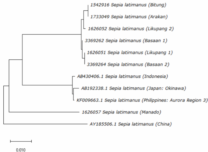
Figure 2. Phylogenetic tree of North Sulawesi S. latimanus .
