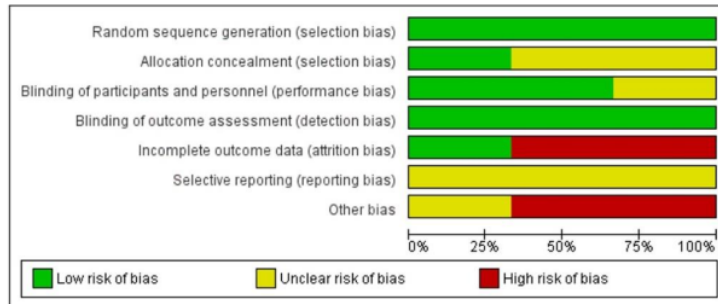
Figure 3. Bias Analysis
