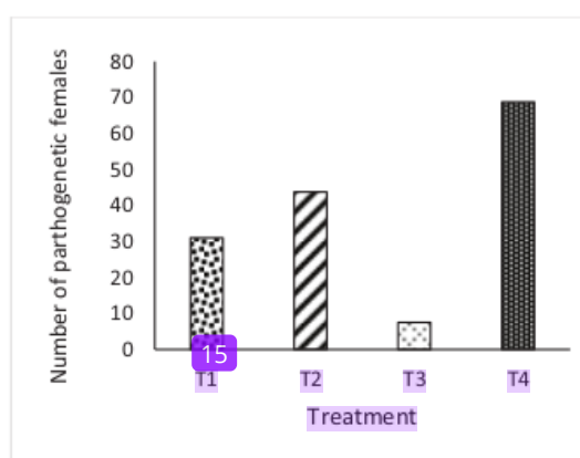
Figure 1. The comparison of each treatment responses on parasite number in the gut of experiment animals
