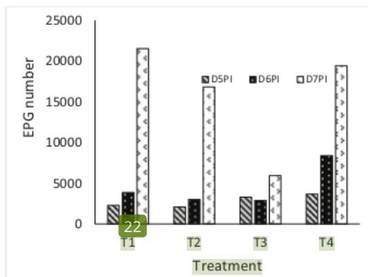
Figure 2. The treatments effect on EPG number. DPI corresponded to 'day post infection'
