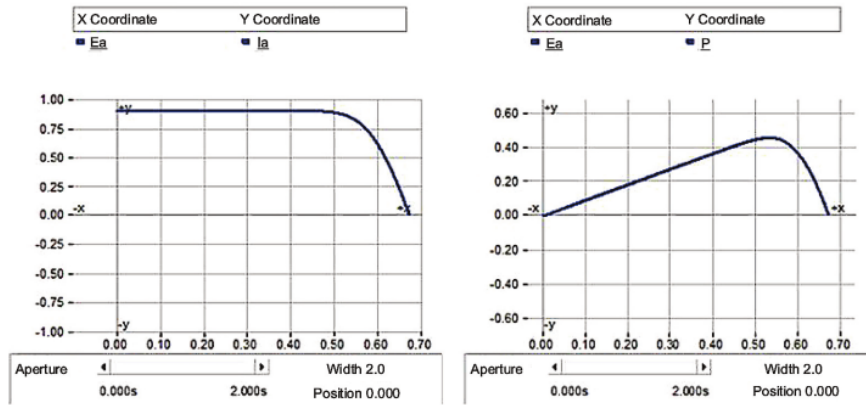
44 Fig. 7. The V - I and P - V characteristics of the PV system.
