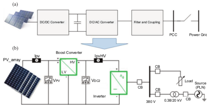
Fig. 1. Grid-connected PV system with a two-stage converter.
