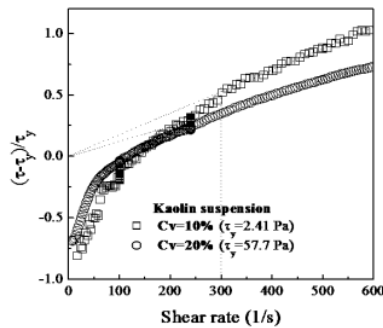
Fig2. Application of Bingham model
