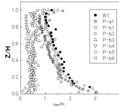
Fig 9. Vertical distribution of u_{rms}/U^*
