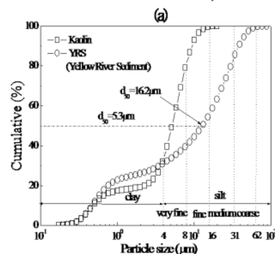
Fig 1. Grain size distributions
