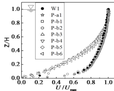
Fig 8. Main flow velocity
