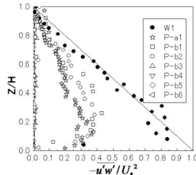
Fig.11 Vertical distribution of -u'w'/U^{*2}
