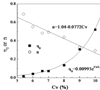
Fig 5. Parameters \eta_0 and n in power-law model
