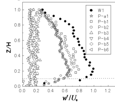
Fig 10. Vertical distribution of w_{rms}/U^*
