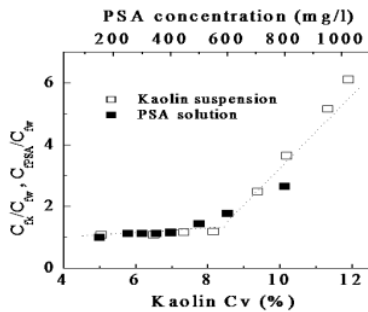
Fig 6. Relationship between flow resistance and concentration
