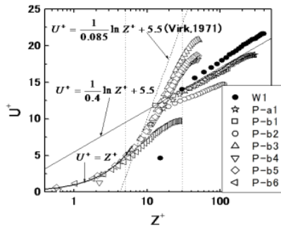
Fig.12. Logarithmic distribution of main flow velocity
