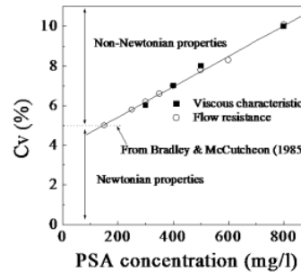
Fig 7. PSA solution equivalent to kaolin suspension
