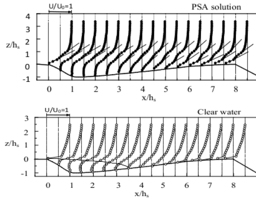
Figure 7. Vertical distribution of main flow velocity
