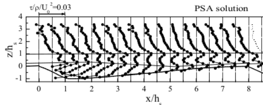
Figure 11. Vertical distribution of viscous stress
