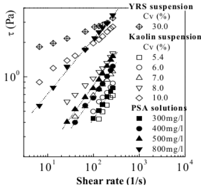
Figure 2. Relation between shear stress and shear rate
