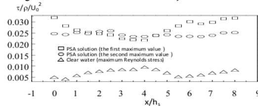
Figure 12. Streamwise distribution of maximum shear stress
