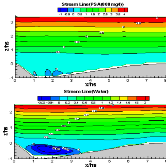
Figure 6. Isolines of a stream function
