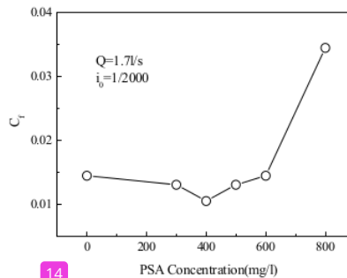
Figure 5. Relationship between the total resistance coefficient and PSA solution
