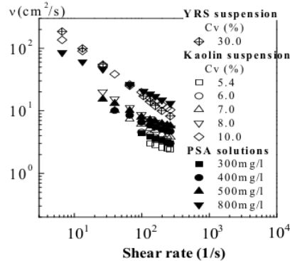
Figure 4. Relation between kinematic viscosity and shear rate
