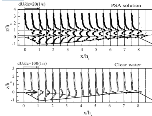
Figure 10. Vertical distribution of shear rate
