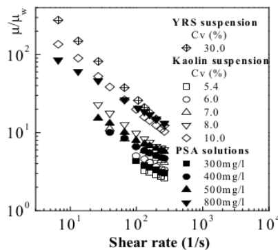
Figure 3. Relation between viscosity and shear rate
