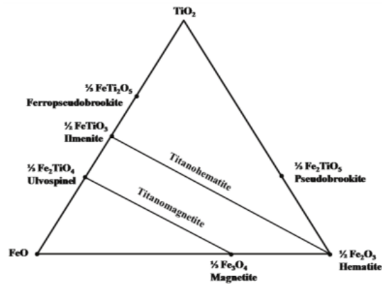
Figure 1. The ternary diagram for the Fe-Ti oxides.
