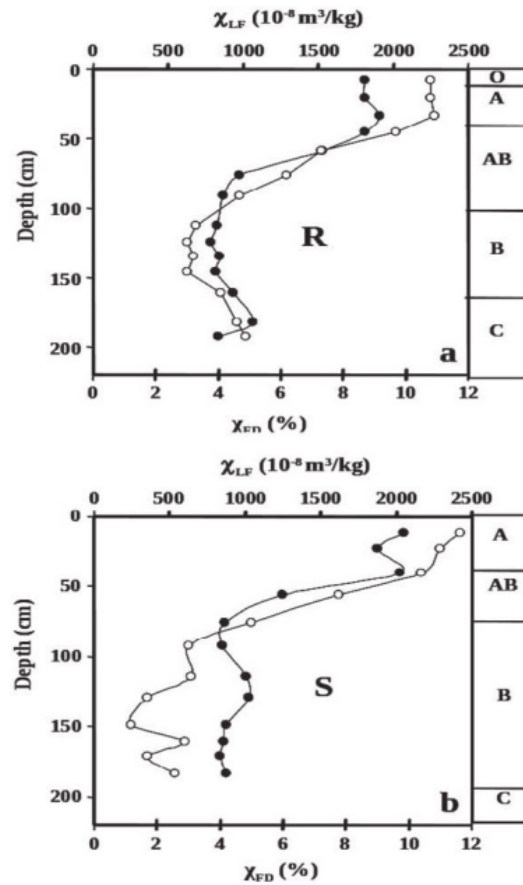
Figure 2. Variation of bulk low frequency magnetic susceptibility ( \chi_{LF} ) and the frequency-dependent susceptibility ( \chi_{FD} (%)) in selected profiles, i.e., profile R (a) and S (b). (Modified from Safiuddin et al. , 2011).
