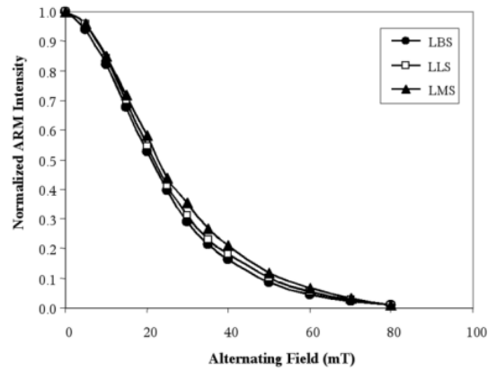
Figure 4 ARM decay curves for cores of LLS, LBS, and LMS.
