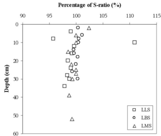
Figure 3 Scattergram of S-ratio showing that magnetite is the predominant magnetic mineral in LLS, LBS and LMS.
