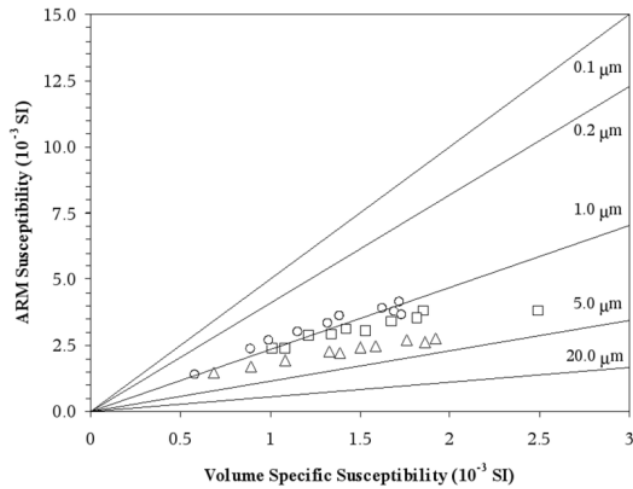
Figure 8 Estimation of magnetite grains size using King's plot ( \square : LLS, \circ : LBS, \Delta : LMS).
