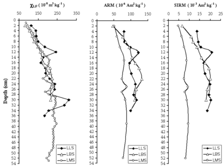
Figure 2 Variation of \chi_{LF} , ARM, and SIRM versus depth for cores from Lakes Lading, Bedali, and Matano.
