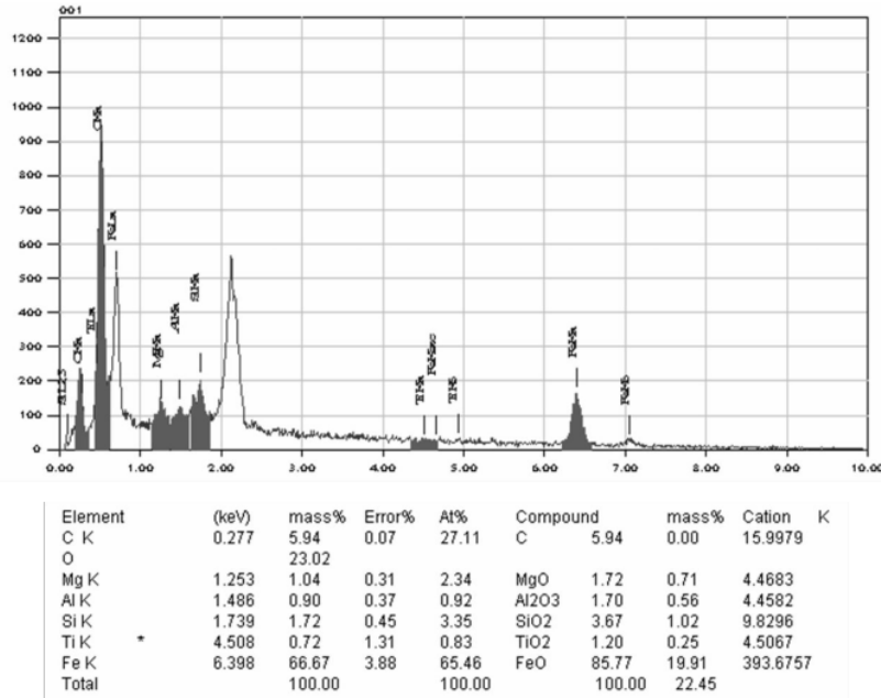
Figure 7 EDX analyses of selected magnetic grain on Lake Matano show high content of FeO and small concentrations of TiO, suggesting largely magnetite or Ti-poor titanomagnetite.
