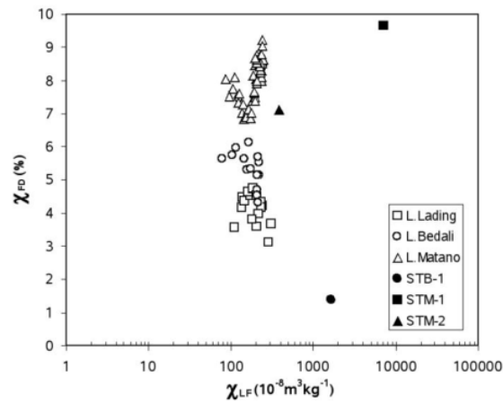
Figure 5 The scattergram of \chi_{FD} -vs- \chi_{LF} showing that different clusters for sediment and soil samples.
