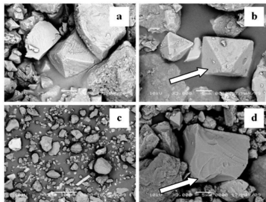
Figure 6 Typical magnetic mineral grains from Lake Bedali (a & b) and Lake Matano (c & d). (a) Detrital magnetic grains with sharp edges, originated from weathered igneous rocks in the volcanic area. (b) Octahedral magnetite with cracks in all parts of the surface (c) BSE image showing the domination of rounded grains; brighter grains indicate higher Fe content (d) A grain with quite significant concentrations of FeO and Chromite ( \text{Cr}_2\text{O}_3 ).
